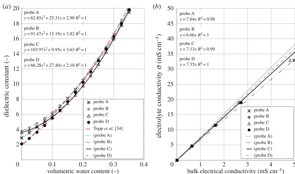
Figure 4. Calibrations for 50 mm long TDR probes: (a) dielectric constant versus with volumetric water content and (b) electrolyte electrical conductivity versus bulk electrical conductivity. (Online version in colour.)
