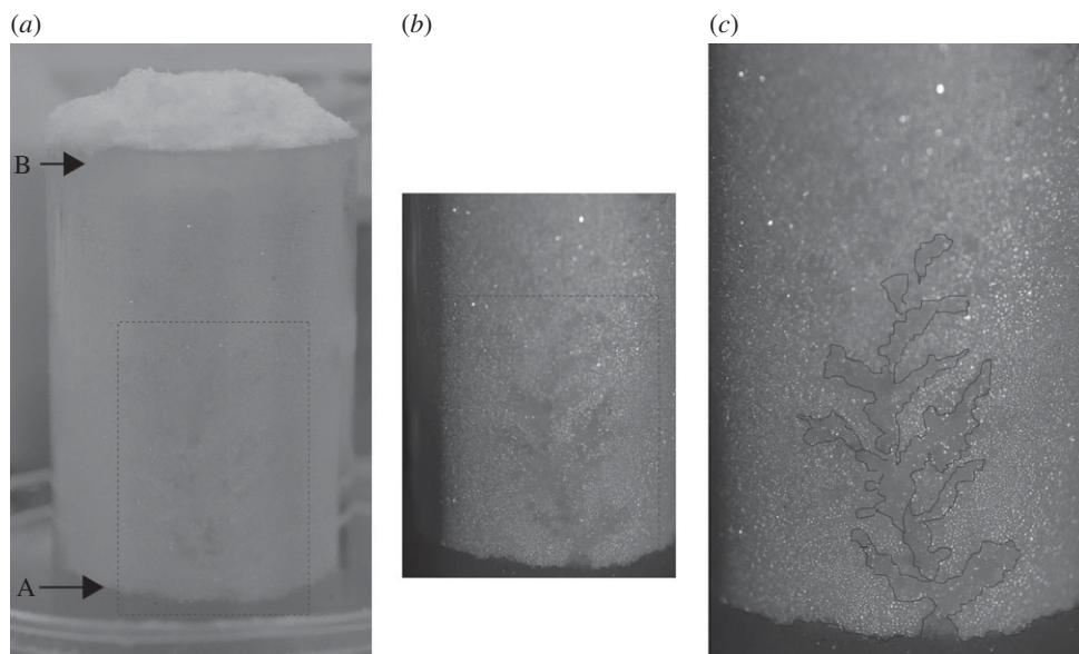
Figure 2. Dendritic migration of salt into dry glass ballotini ( 600\text{--}425\text{ }\mu\text{m} ). (a) Showing dendrite above the capillary fringe (A) with raised surface capped by salt (B), (b) close-up of dendrite, (c) outline of dendrite accentuated.
