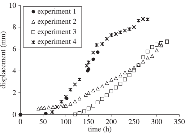
Figure 7. Surface displacement caused by salt heave.
